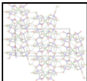
Fig. 2. Crystal packing of title compound, projection down the b axis. Dashed lines indicate hydrogen bonds.
